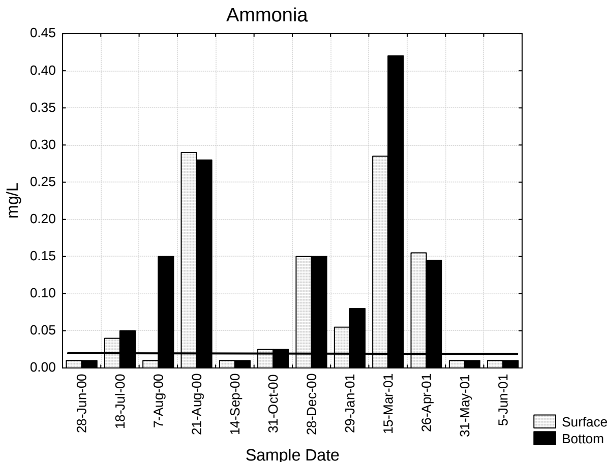
Figure 22. Average surface and bottom concentrations of total ammonia by sample date for Cresbard Lake. Line is detection limit (0.02 mg/L).
