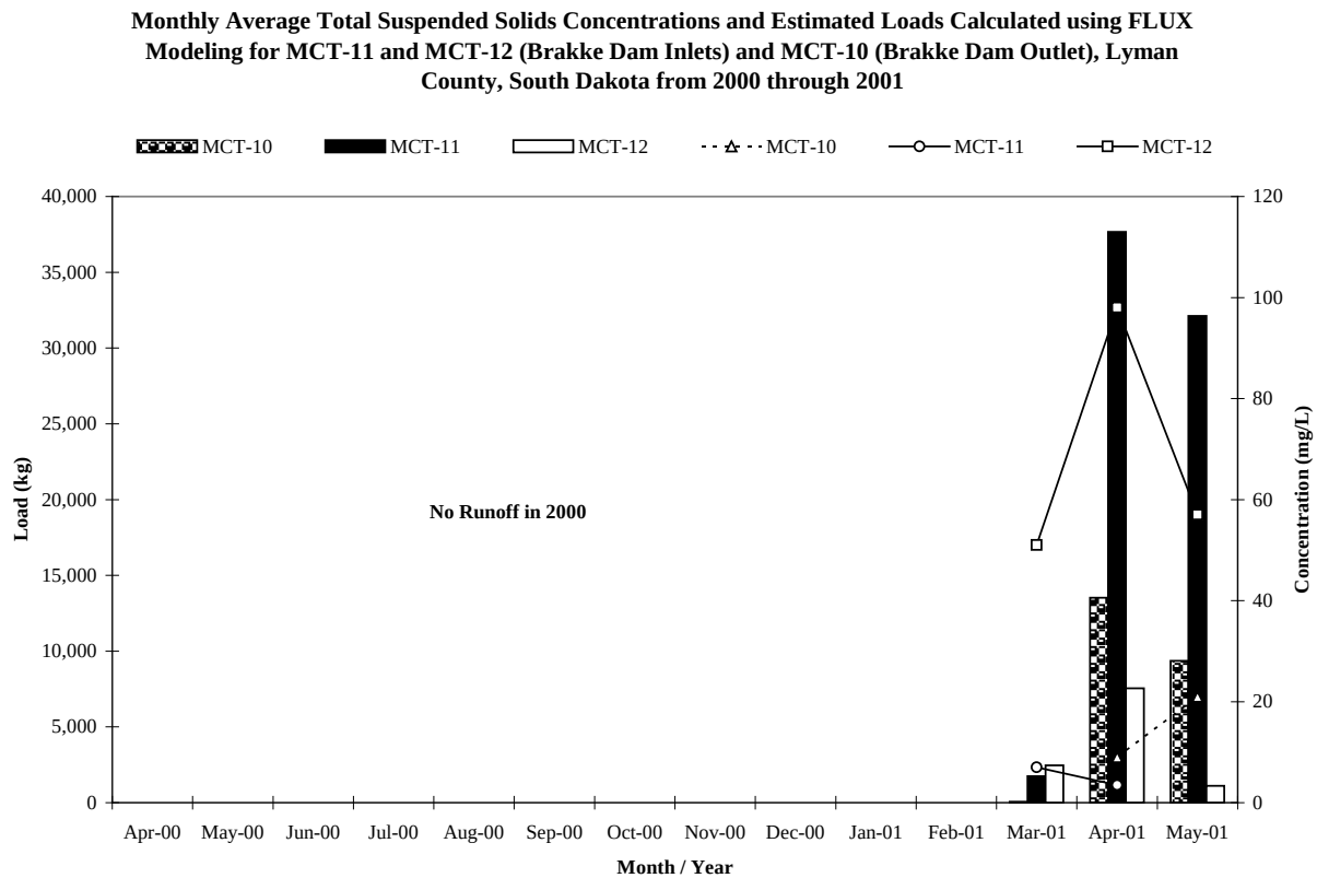
Figure 12. Monthly average total suspended solids concentrations and estimated loads by tributary to Brakke Dam and Medicine Creek from Brakke Creek, Lyman County, South Dakota from 2000 through 2001.
