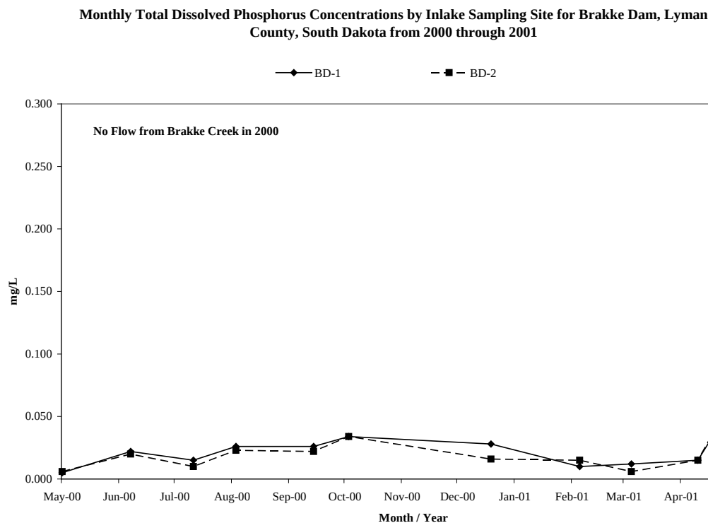
Figure 45. Monthly surface total dissolved phosphorus concentrations by date and sampling site for Brakke Dam, Lyman County, South Dakota from 2000 through 2001.
