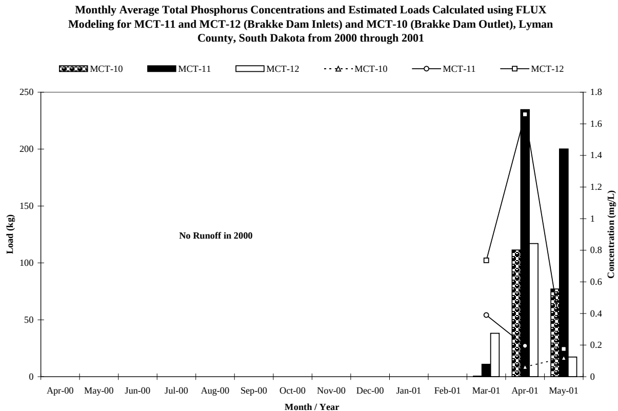
Figure 21. Monthly average total phosphorus concentrations and estimated loads to Brakke Dam and Medicine Creek from Brakke Creek, Lyman County, South Dakota from 2000 through 2001.
