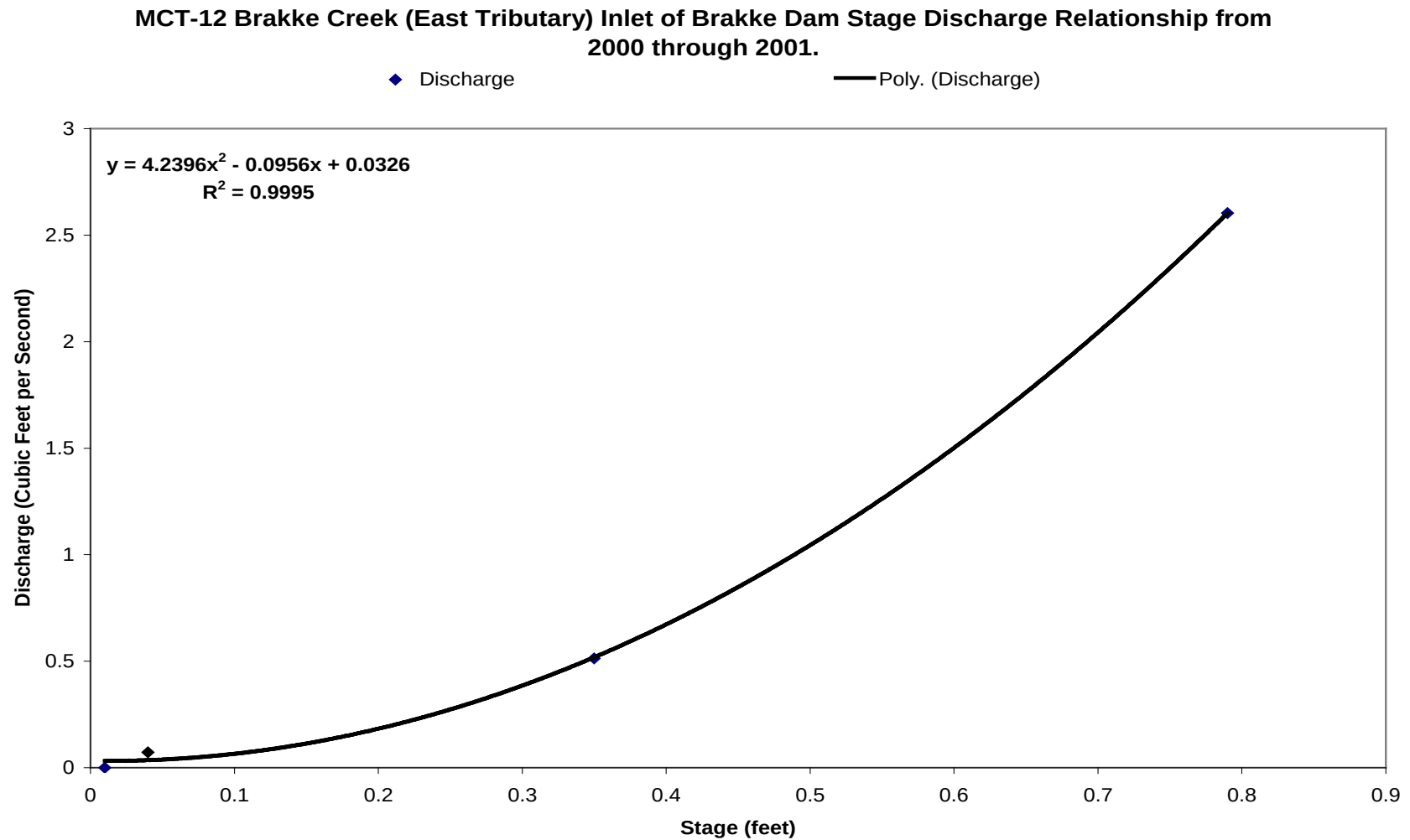
Figure A1. Stage discharge relationship for MCT-12 (east tributary of Brakke Creek) from 2000 through 2001.
