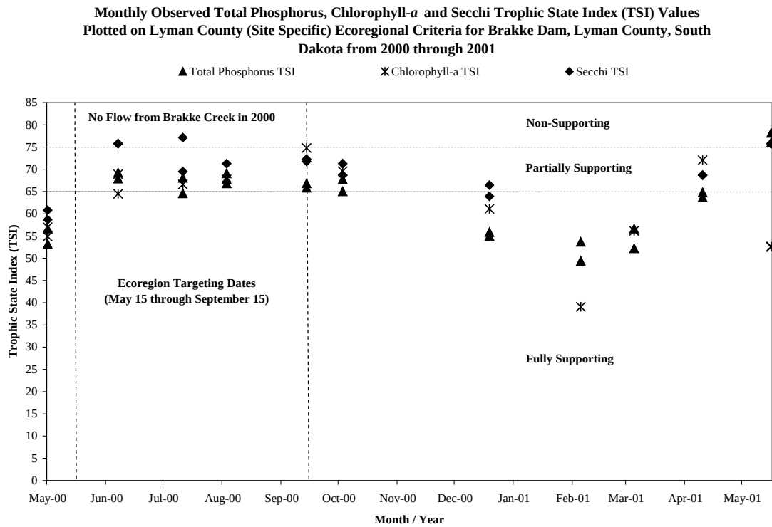
Figure 58. TSI values for phosphorus, chlorophyll- a and Secchi TSI plotted by proposed Lyman County (site specific) beneficial use categories for Brakke Dam, Lyman County, South Dakota by date in 2000 and 2001.
