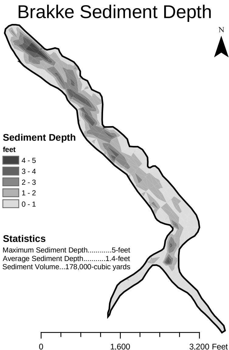
Figure 70. Sediment survey sediment depth for Brakke Dam, Lyman County, South Dakota for January 2002.
