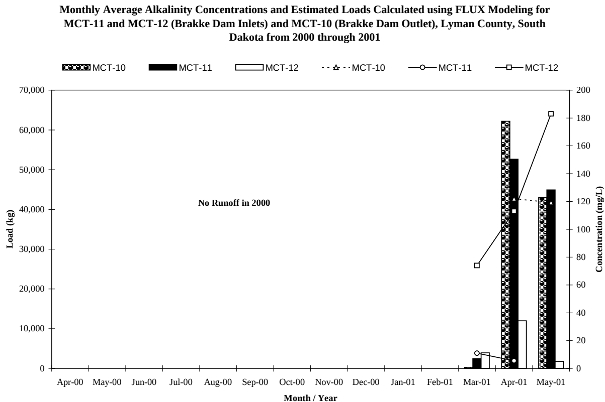
Figure 8. Monthly average total alkalinity concentrations and estimated loads by tributary to Brakke Dam and Medicine Creek from Brakke tributaries and Brakke outlet, Lyman County, South Dakota in 2000 and 2001.
