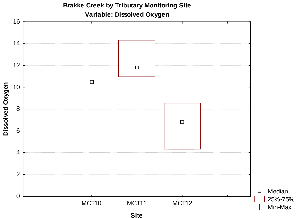
Figure 5. Median, quartile and range for dissolved oxygen concentrations by tributary monitoring site for Brakke Creek, Lyman County, South Dakota from 2000 through 2001.
