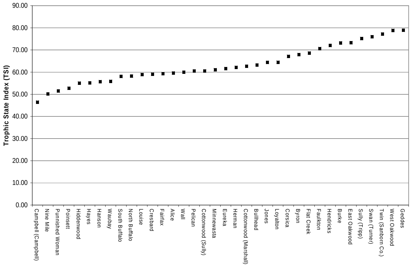
Median Secchi-Chlorophyll-a Trophic State Index (TSI) for Assessed Lakes Designated for Warmwater Semi-Permanent Fish Life Propagation: 2000-2009
