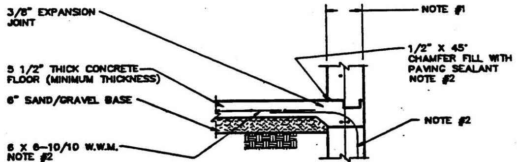
WALL TO SLAB SECTION
