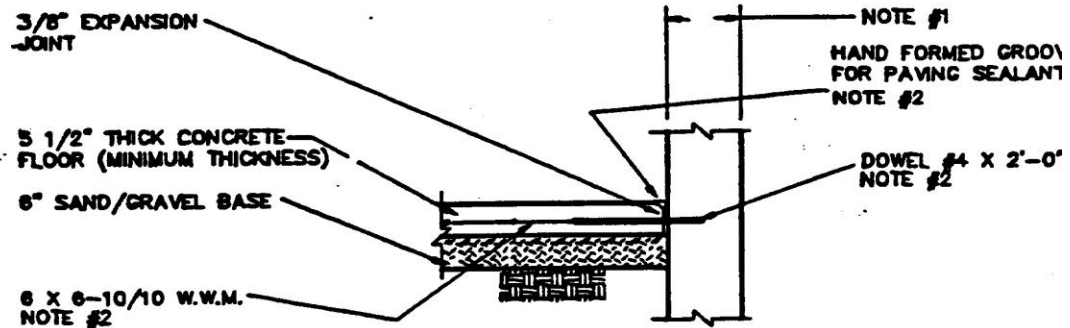
SLAB TO WALL SECTION
