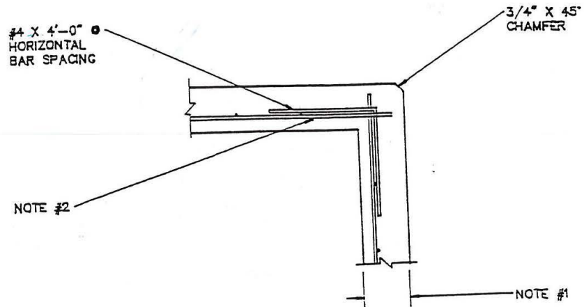
CORNER PLAN DETAIL
