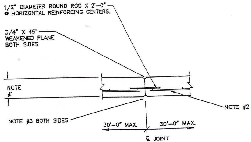
WALL JOINT PLAN DETAIL
