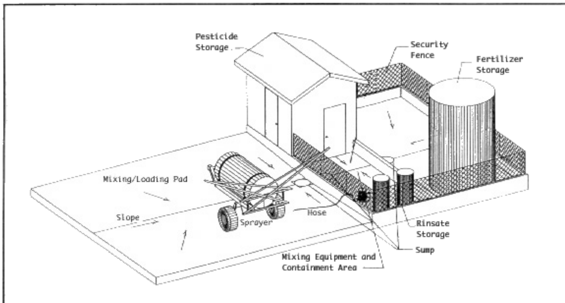
Combination mixing and storage area for pesticide and fertilizer handling.
